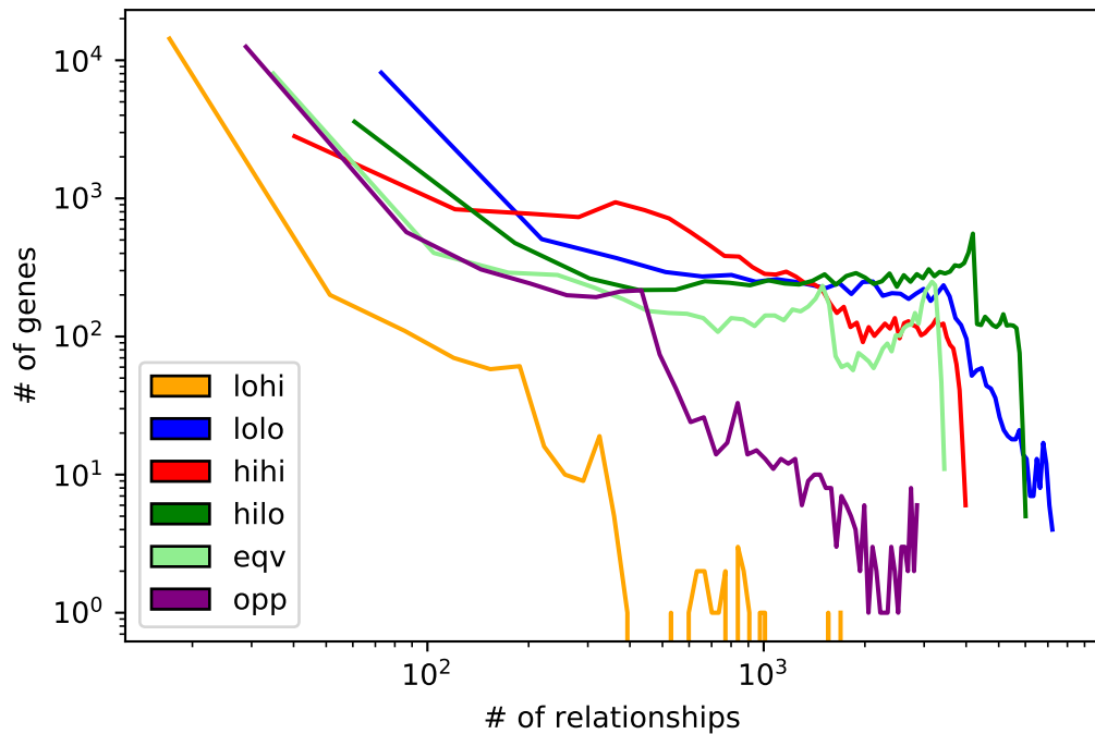
GSE98556, n = 546
